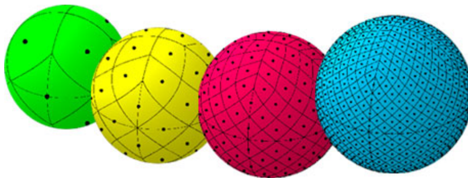
Fig. 4: An illustration of the first four HEALPix tessellations ( n_{\text{side}}=1 , n_{\text{side}}=2 , n_{\text{side}}=4 , and n_{\text{side}}=8 ). Reproduced from https://healpix.jpl.nasa.gov .
