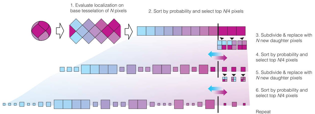
Fig. 1: An illustration of the adaptive mesh refinement scheme, reproduced from Page 64, 1 .
