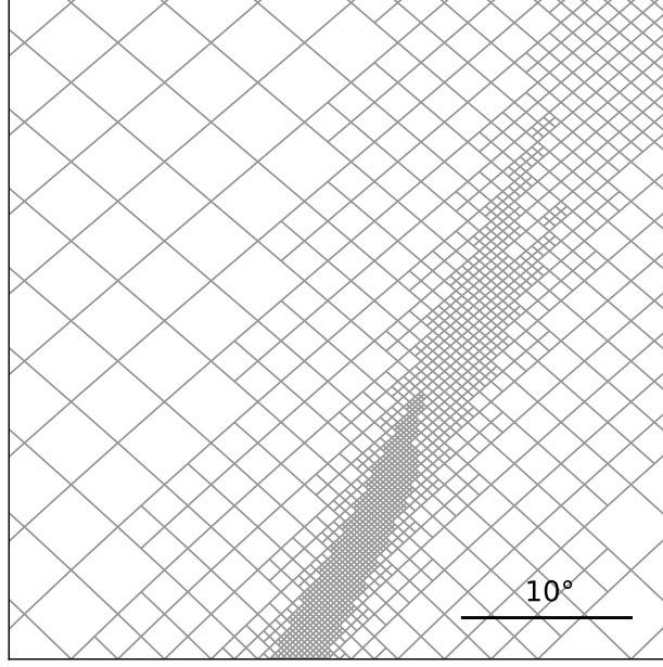
Fig. 2: An example multi-resolution mesh from a typical two-detector ( LHO and LLO ) localization produced with BAYESTAR. Reproduced from 1 . The scale bar at bottom right has a length of 10°.
