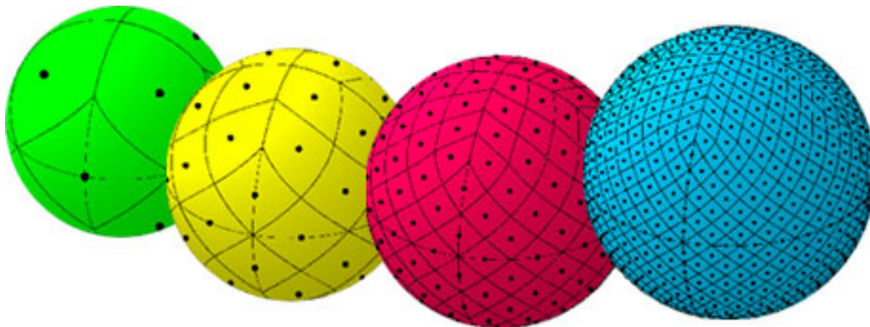
Fig. 1: An illustration of the first four HEALPix tessellations ( n_{\text{side}}=1 , n_{\text{side}}=2 , n_{\text{side}}=4 , and n_{\text{side}}=8 ). Reproduced from https://healpix.jpl.nasa.gov .
